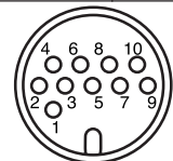
Figure A-1 — LDT Pin Diagram
